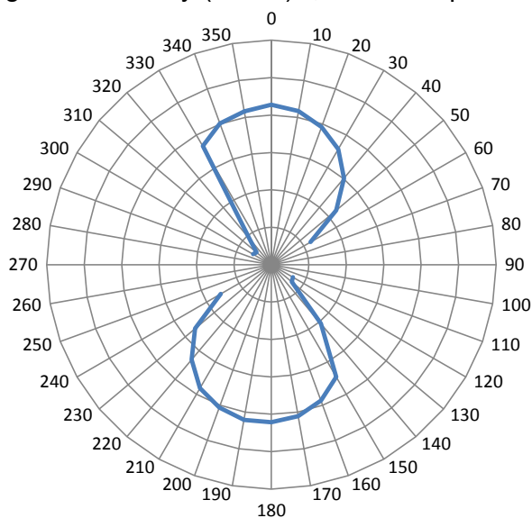
Angular Sensitivity (Relative Read Range vs. Orientation)
