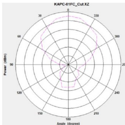
Radiation Pattern
