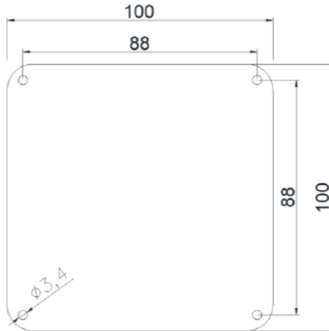
Antenna Drawing
